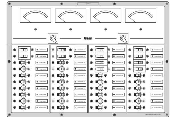
90-9180 19"W x 13.5"H x 3.5"D
