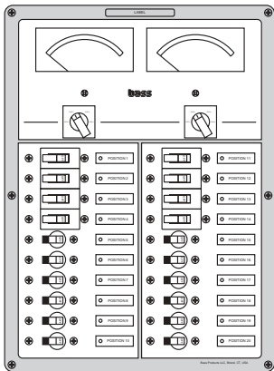
90-9160 10"W x 13.5"H x 3.5"D
