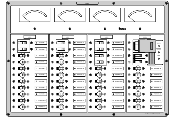
90-9140PS* 19"W x 13.5"H x 3.5"D * Shown with optional sliding interlock which is available on all models
