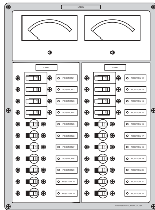
90-9120 10"W x 13.5"H x 3.5"D
