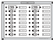
90-9124 10"W x 7.5"H x 3.5"D
