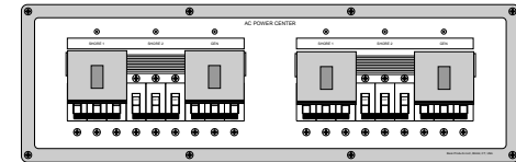
90-9445 19"W x 6"H x 3.5"D
