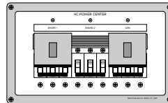
90-9425 10"W x 6"H x 3.5"D
