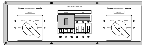
90-9340 19"W x 6"H x 3.5"D
